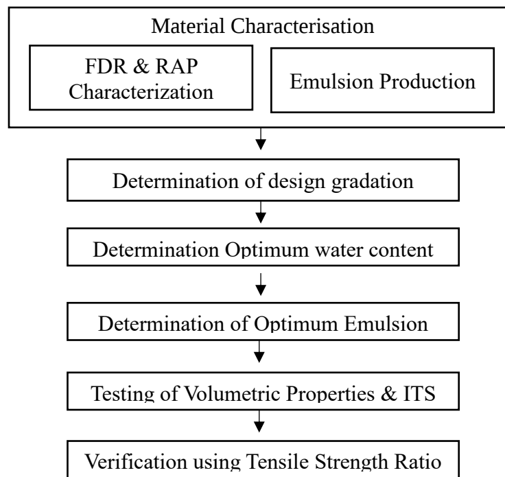
Fig 5: Steps included in the mix design of AEFDR
